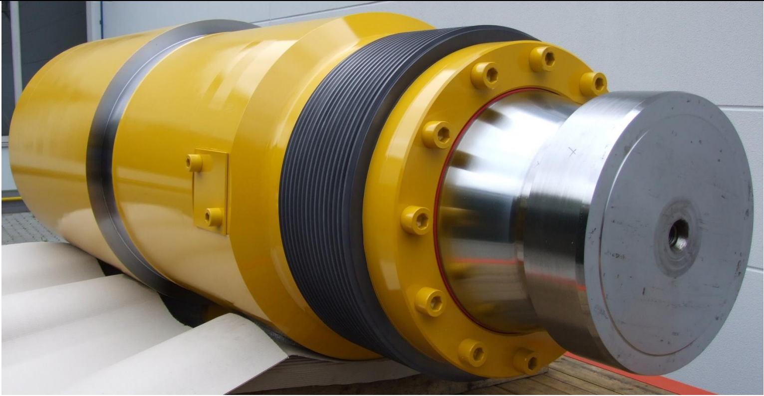
Hydraulic cylinder, piston diameter 710 mm, rod diameter 530 mm, stroke 1250 mm, weight 16200 kg
