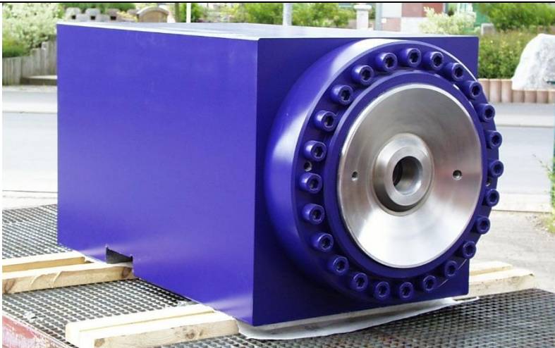
Hydraulic cylinder, piston diameter 675 mm, rod diameter 645 mm, stroke 500 mm, weight 9900 kg
